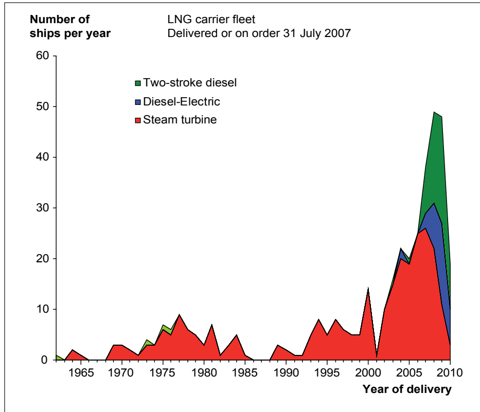
Fig. 5b: Distribution of propulsion systems of LNG fleet in year of delivery
