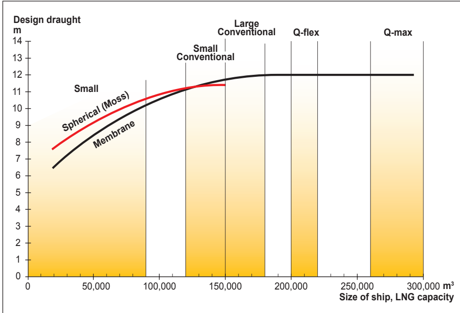
Fig. 9: Average design draught of LNG carriers (membrane and Moss types)
