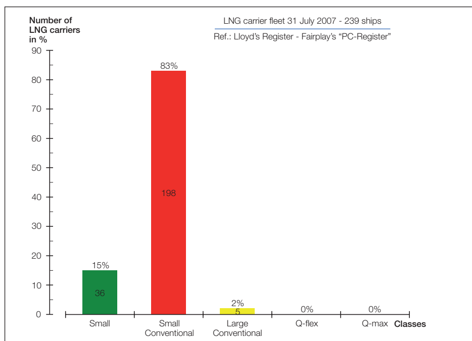
Fig. 4a: Distribution of existing LNG carriers in service (number of ships)
