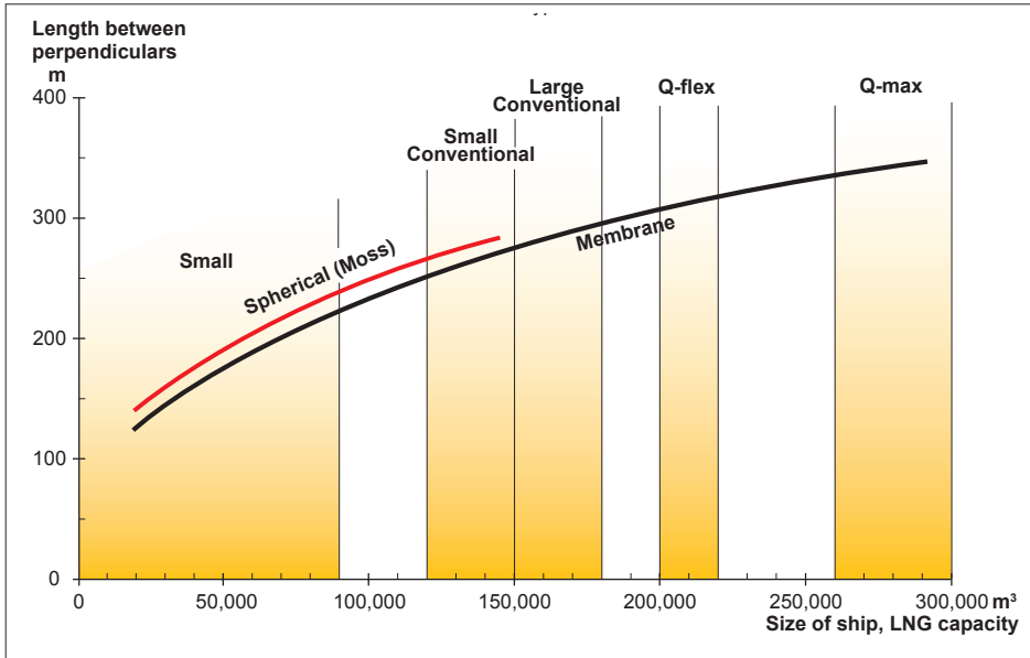
Fig. 7: Average length between perpendiculars of LNG carriers (membrane and Moss types)
