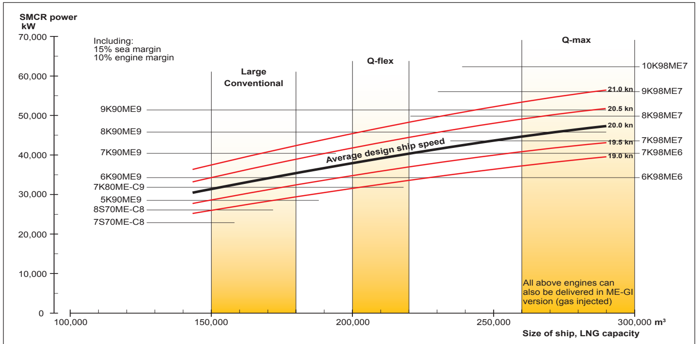
Fig. 15: Propulsion SMCR power demand of an average LNG carrier (membrane type), Large Conventional, Q-flex and Q-max – single-screw
