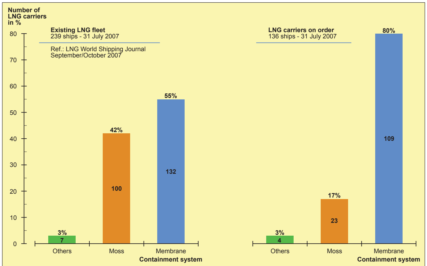
Fig. 2: Distribution in containment systems on LNG fleet
