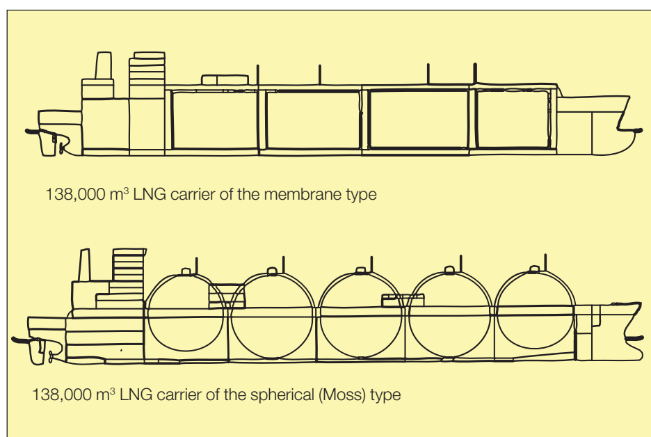
Fig. 1: Examples of equal-sized LNG carriers based on the membrane and the spherical (Moss) types shown in the same scale
