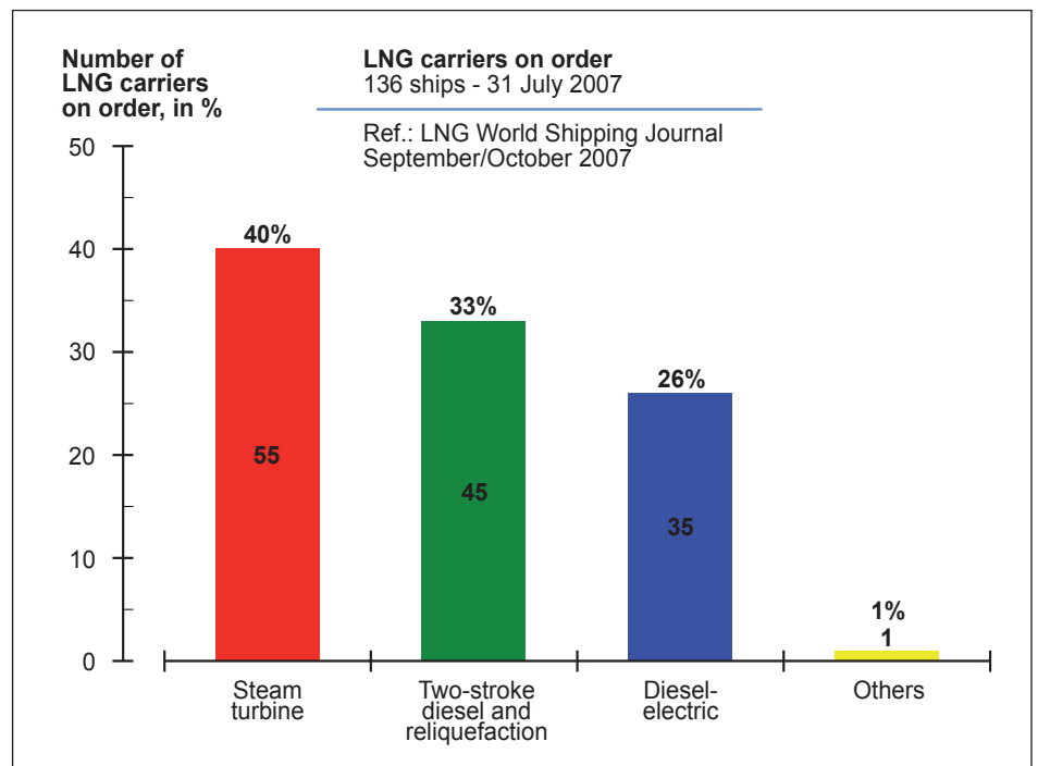
Fig. 5a: Distribution of propulsion systems of LNG fleet on order
