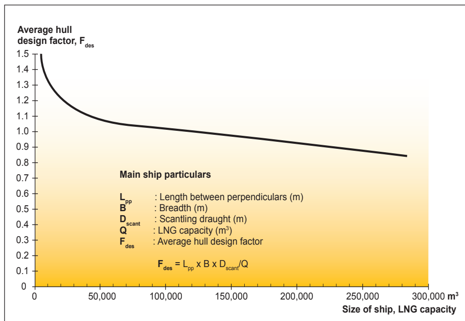
Fig. 6: Average hull design factor of LNG carriers (membrane type)
