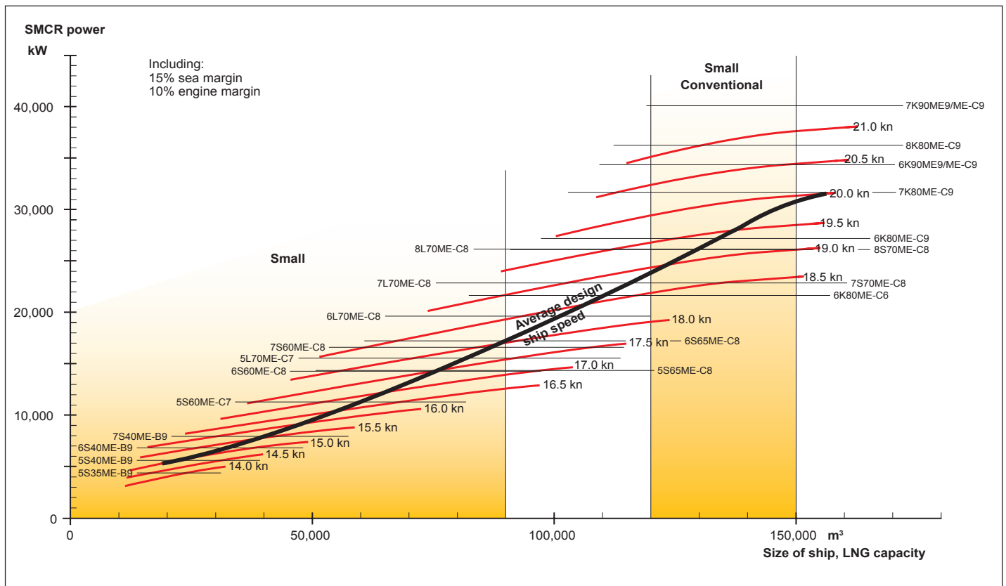
Fig. 14: Propulsion SMCR power demand of an average LNG carrier (membrane type), Small and Small Conventional – single-screw
