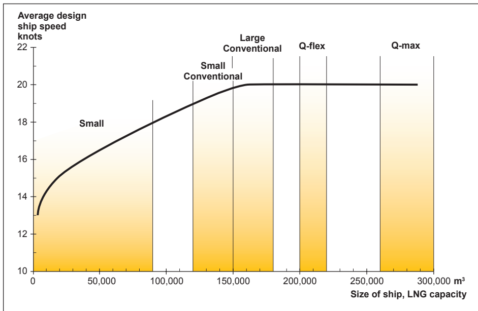
Fig. 10: Average design ship speed of LNG carriers
